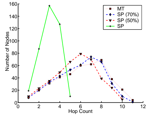
(a) Hop Distribution
