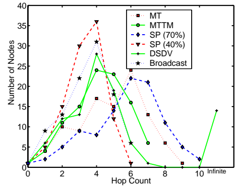
Figure 8: Hop distribution from simulations.
